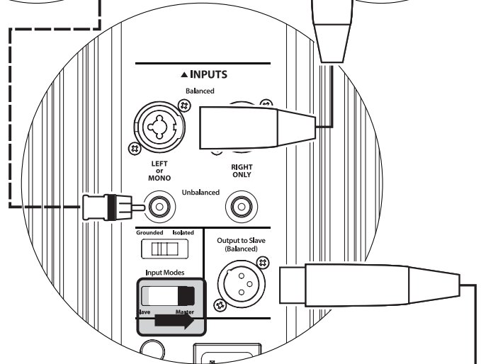
GOTHAM REAR CONTROLS (MASTER)
