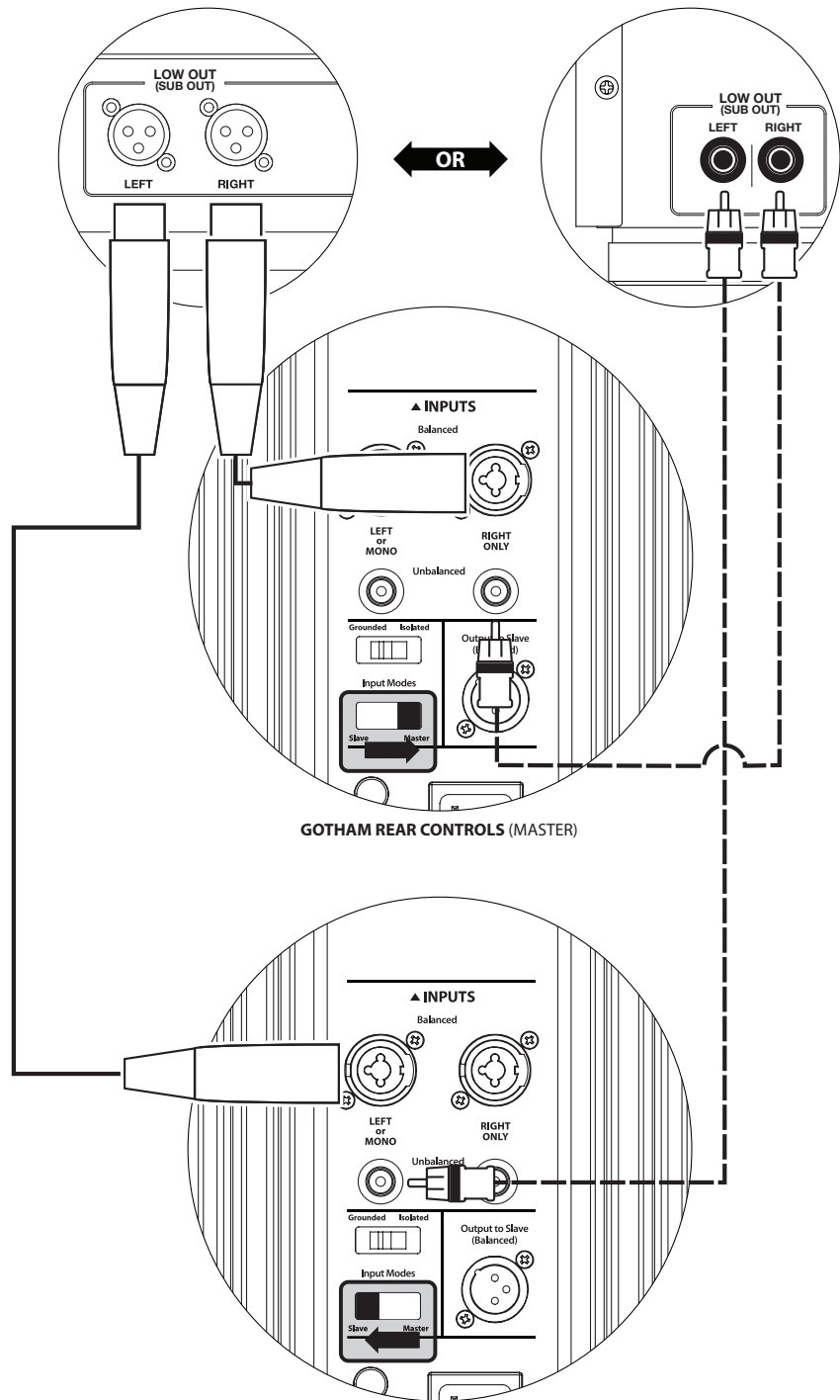
STEREO ACTIVE CROSSOVER (BALANCED OUTPUTS)
