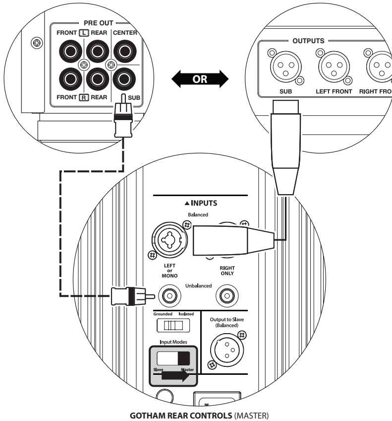
GOTHAM REAR CONTROLS (MASTER)
